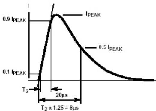
FIGURE 3B. DISCHARGE CURRENT WAVEFORM FIGURE 3. UNIDIRECTIONAL WAVESHAPES (OUTDOOR LOCATIONS)
